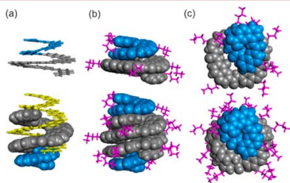
Figure 2. Side (a,b) and top (c) views of energy-minimized models of single helical 2 and double helical ( 2 ) 2 . Aromatic backbones are color coded in blue (quinoline) and gray (fluoroquinoline). In (a), one strand of ( 2 ) 2 is shown in a yellow tube representation. Side chains were omitted for clarity. In (b) and (c), 2 and ( 2 ) 2 are shown as CPK models. Side chains are shown as purple tubes.
