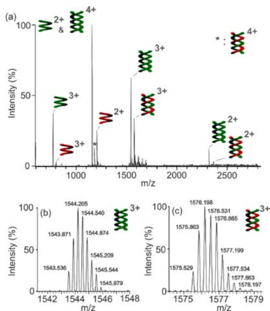
Figure 4. (a) Electrospray ionization mass spectrum (ESI-MS) of a solution of 20 \mu\text{M} of oligomer 2 in water. The homoduplex of 2 (green helices) and heteroduplex of 2 –COCF _3 (red helices) are detected. Excerpts of the high resolution ESI mass spectrum of: (b) the homoduplex ( 2 ) _2 and (c) the heteroduplex 2 – 2 –COCF _3 .
