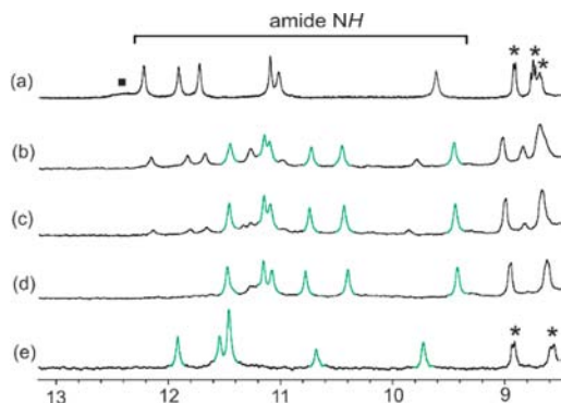
Figure 3. Excerpts of the ^1\text{H} NMR (400 MHz) titration at 298 K of 1 (2 mM) in DMSO- d_6 /H _2 O mixtures in the following vol/vol ratios: (a) 100:0; (b) 80:20; (c) 76:24; (d) 70:30. (e) ^1\text{H} NMR (400 MHz) spectrum of ( 1 ) _2 in water (H _2 O/D _2 O 90:10 vol/vol). Black and green signals stand for single and double helix, respectively. Some aromatic resonances are denoted with stars. The signal of the carboxylic acid is marked with a black square.
