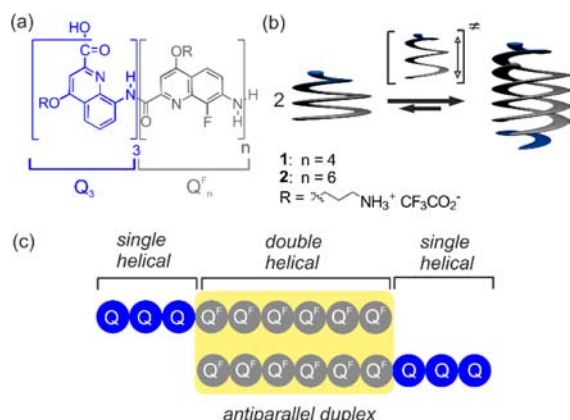
Figure 1. (a) Formula of 1 and 2 ; (b) schematic representation of a single-helix–double-helix equilibrium requiring springlike extension; (c) simplified representation of double helix ( 2 ) 2 . Quinolines are denoted in blue, whereas fluoroquinolines are shown in light gray.
